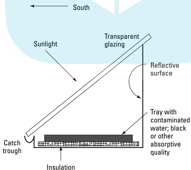
Figure 10-5: A cross-section of a solar still, or water purification system.
